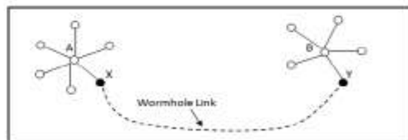
Fig. 3. Wormhole Attack
