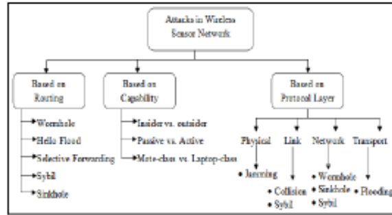
Fig. 2. Attacks Classification in WSN
