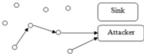
Fig. 5. HELLO Flood Attack scenario-Sensor node replying back to the attacker considering it as its neighbor node
