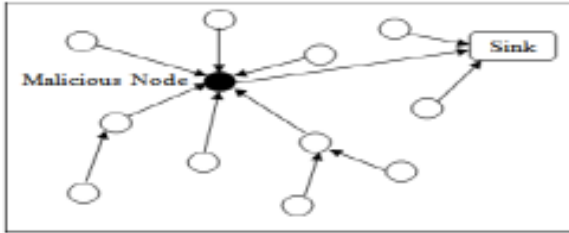
Fig. 8. Sinkhole Attack
