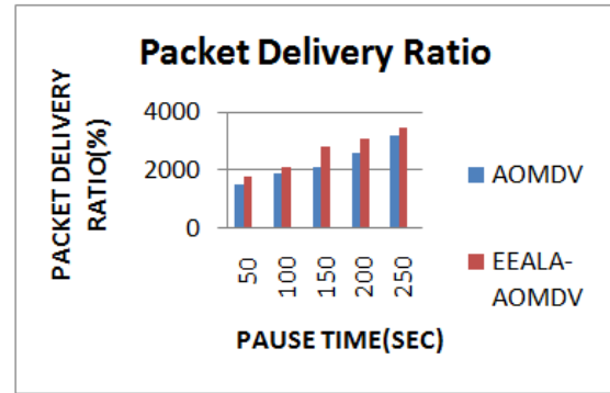
Figure 5 Pause Time Vs Packet Delivery Ratio (%)
