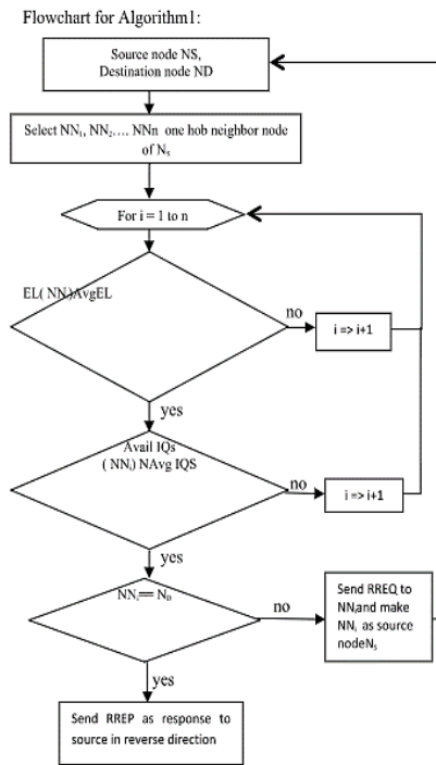
Figure 1 Flowchart-EEALA-AOMDV
