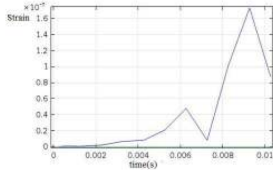
Figure 6: Strain plot for single point load using edge point probe.
