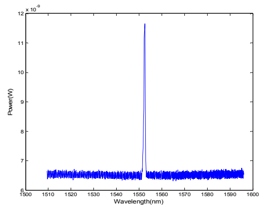
Figure 15: FBG reflected spectrum for 0.348 \mu\epsilon
