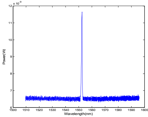
Figure 16: FBG reflected spectrum for 1.392 \mu\epsilon
