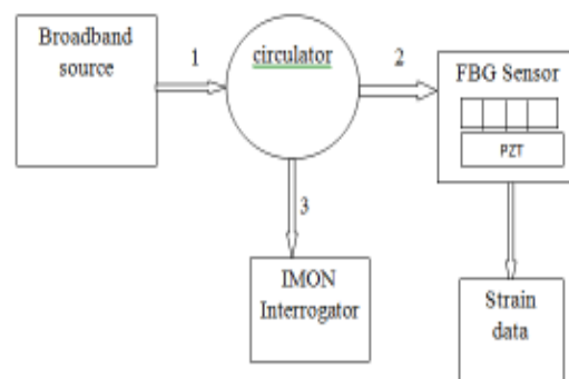
Figure 1: Experimental setup for determination of Bragg wavelength shift.
