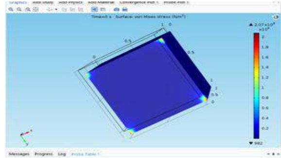
Figure 10: Strain creation-3Dmodel
