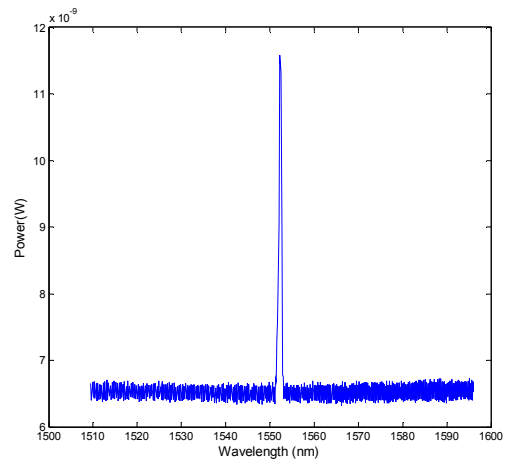
Figure 14: FBG reflected spectrum without strain
