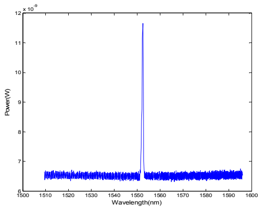
Figure 17: FBG Reflected spectrum for maximum strain
