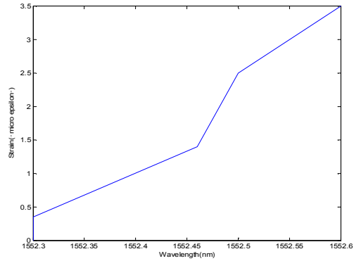
Figure 18: Bragg wavelength at maximum strain
