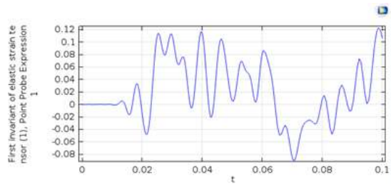
Figure 6: Strain plot for single point load using edge point probe.
