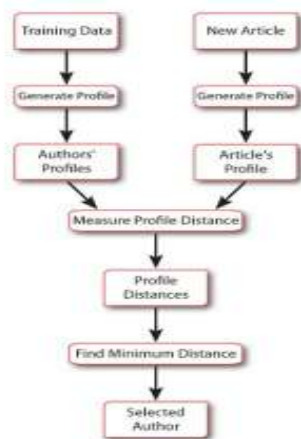
Figure.3.N-gram based Text Classification
