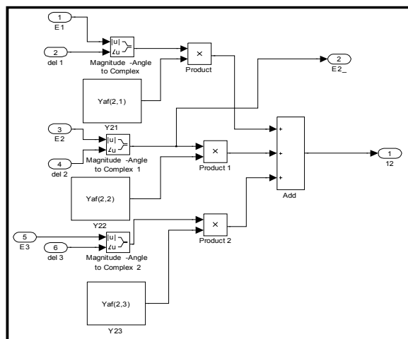
Figure 3: Subsystem 1.
