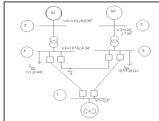
Figure 1: Multi-machine test system under consideration.
