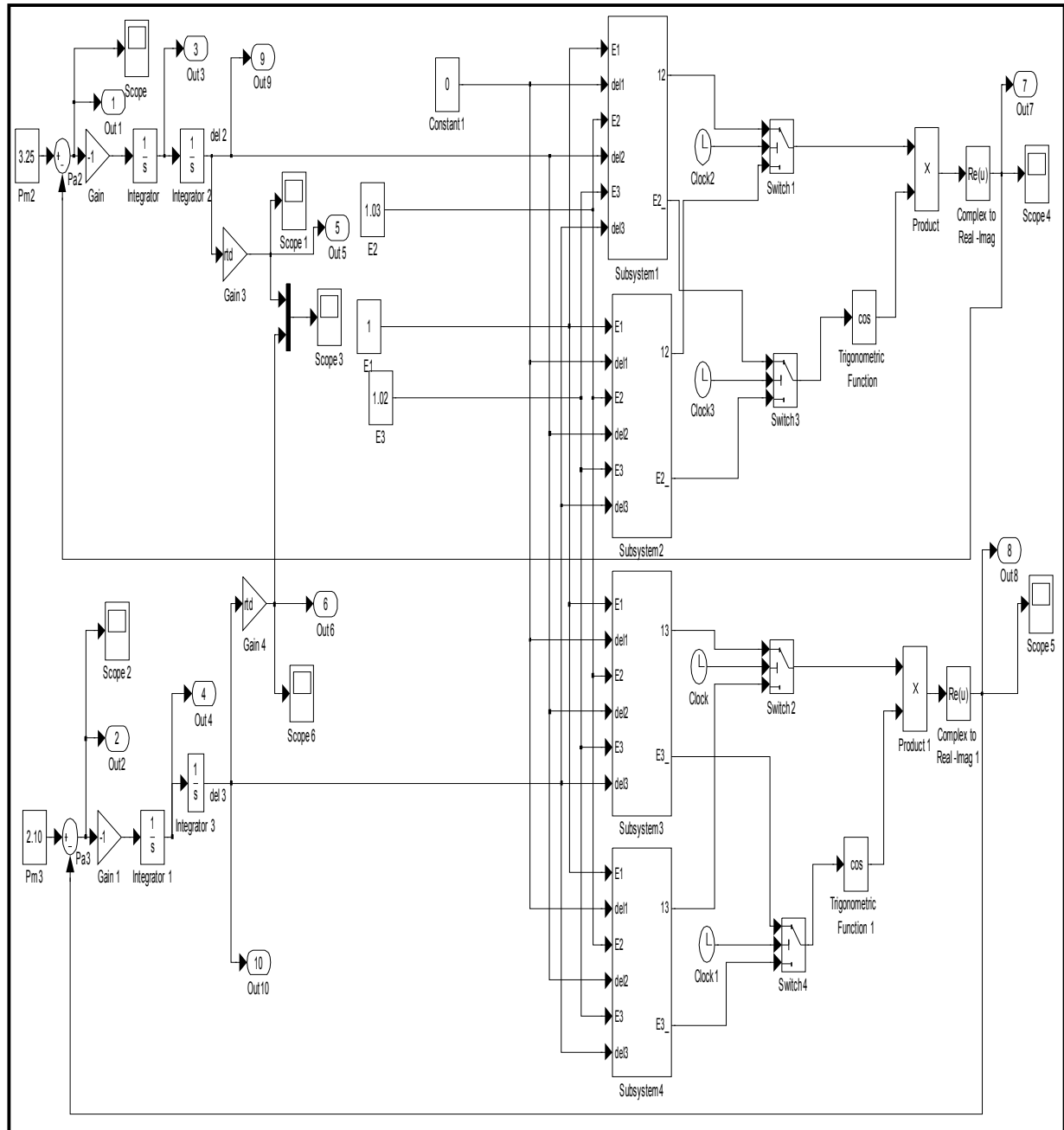
Figure 2: Complete block diagram of the system for transient stability study.
