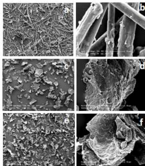
Figure 6: a, b: 1hr treated MFC, c, d : 10hrs treated MFC, e, f: 24hrs treated MFC
