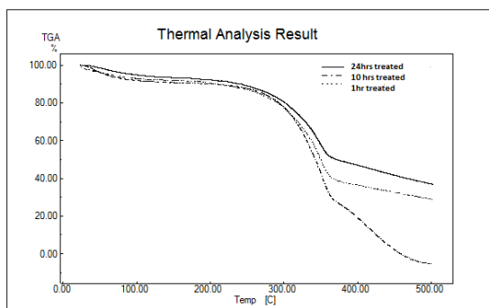
Figure 5: Thermo-gravimetric Analysis (TGA)
