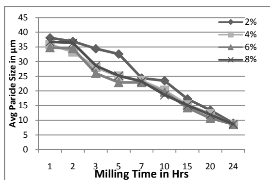
Figure 2: Effect of Milling Time on Particle Size Of MCF
