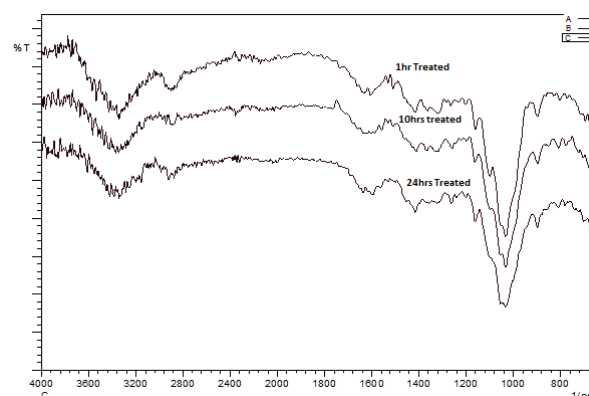
Figure 3: FTIR spectra of Isolated MFC Analysis
