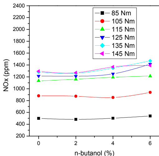
Figure 5: Variation of NO x emission for various butanol percentages at 3000 rpm and 1500 rpm respectively.
