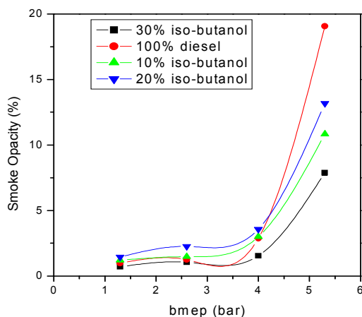
Figure 7: Variation of Smoke Opacity for pure diesel and various percentages of iso-butanol blend.
