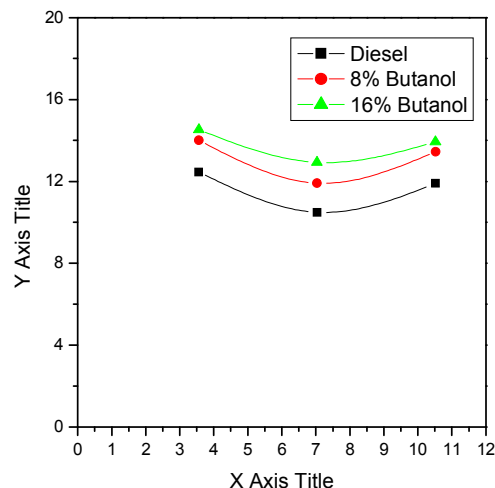
Figure 6: Variation of HC emission for various butanol percentages at 1200 rpm and 1500 rpm respectively.
