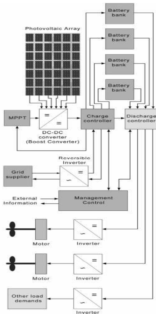
Figure 3.2 Topology of solar-electric boat
