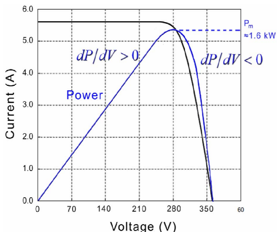
Figure 3.1: Output characteristic curve of photovoltaic array strings.
