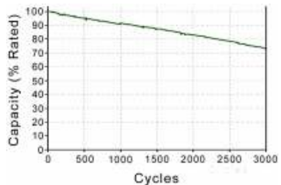
Figure 3.1: Valence U27-36XP capacity retention
