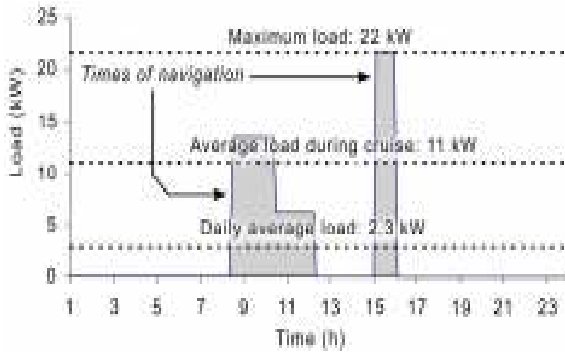
Figure 2.2: Daily load
